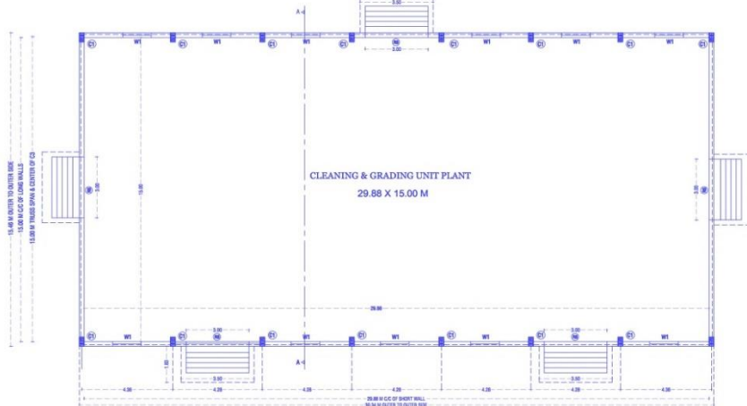
CLEANING & GRADING UNIT PLANT PLAN
