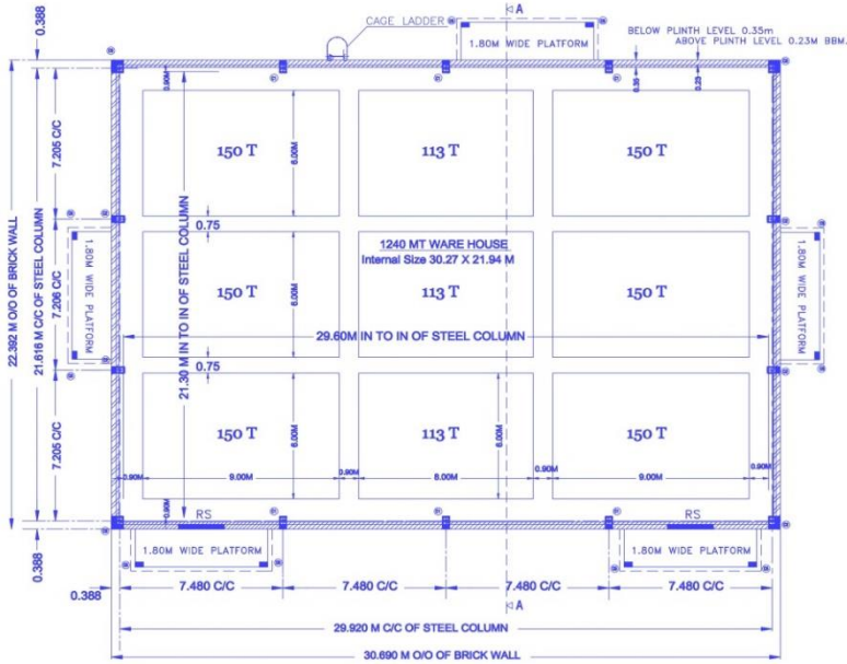
PLAN FOR 1240 MT WARE HOUSE UNIT
